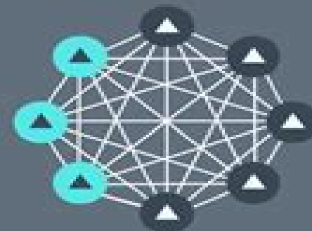
BOLTZMANN MACHINE
