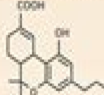
Tetrahydrocannabivarin carboxylic acid THCVA
