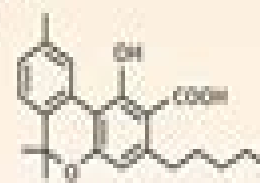
Cannabinolic acid CBNA
