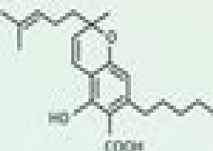
Cannabichromenic acid CBCA
