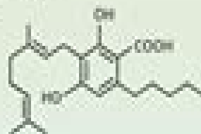
Cannabigeronic acid CBGA
