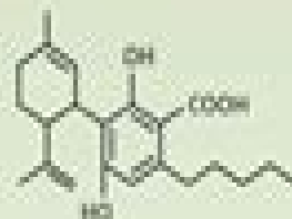
Cannabidiolic acid CBDA
