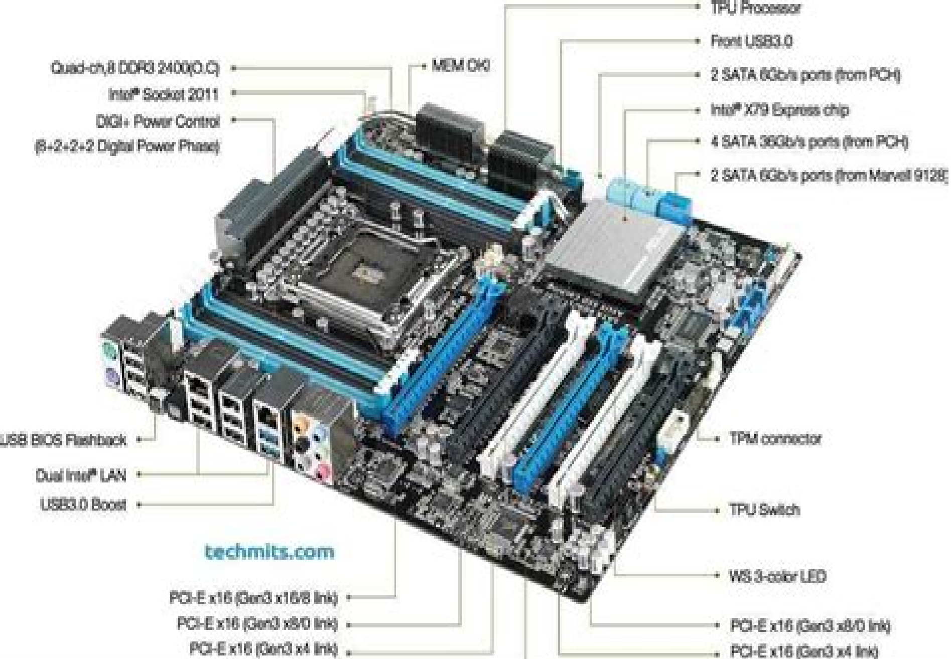
Block Diagram of (Parts/Components) Motherboard
