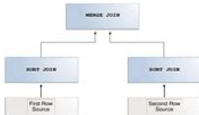
Figure 9-6 Sort Merge Join
