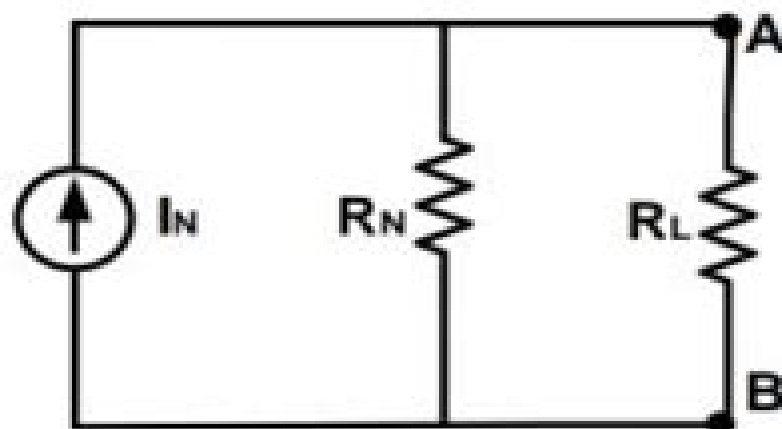
Figure-3.2: Norton equivalent circuit
