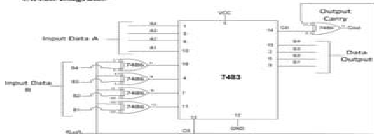
4-BIT Parallel Adder Using 7483 where S=0
