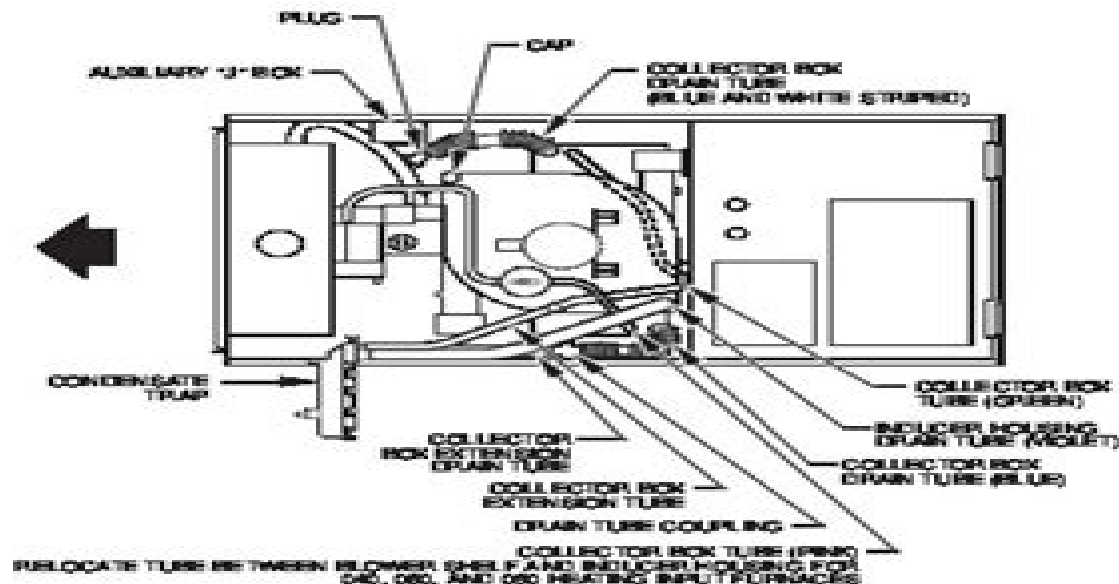
Fig. 10—Horizontal Left Tube Configuration
