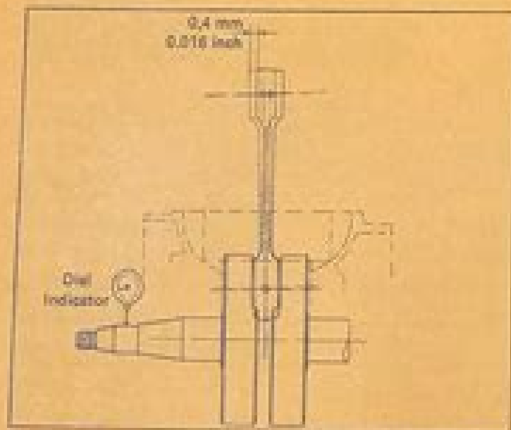
Fig. 15 - Checking connecting rod small end swing and flywheel trueness
