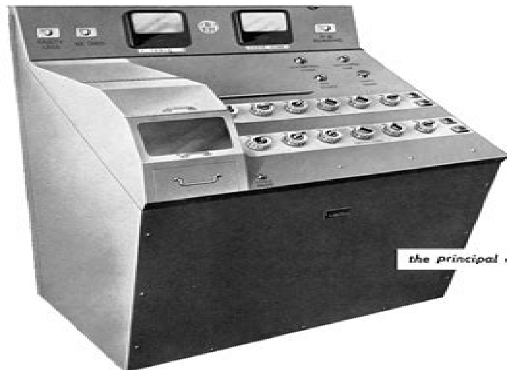
B.T.H. desk with controls for co-ordinate setting and punched card operation.
