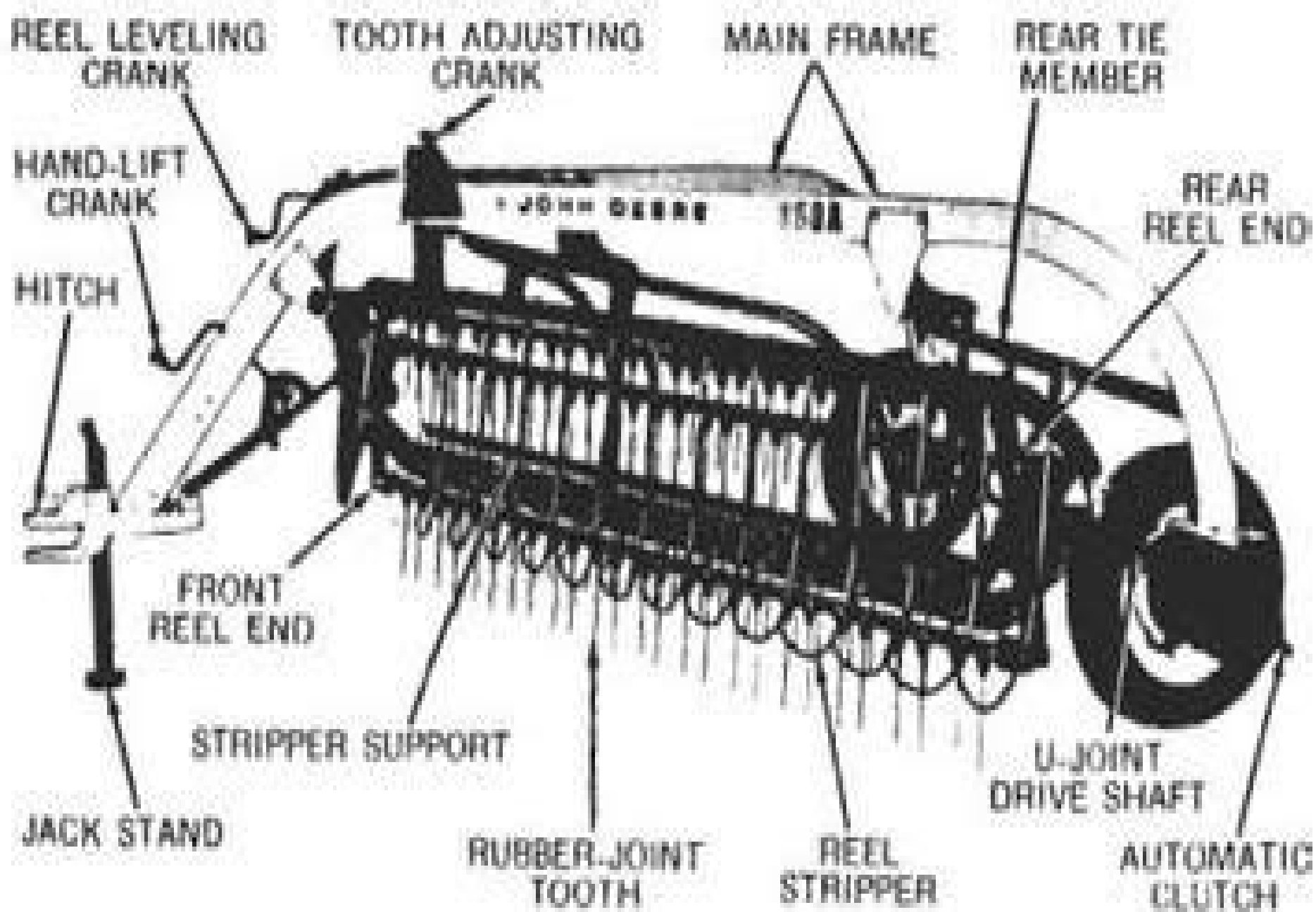
Left-hand side view of John Deere 858A side-delivery rake
