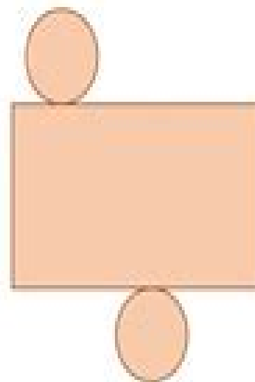
Net of a cylinder
