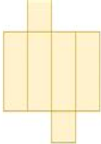
Net of a cuboid
