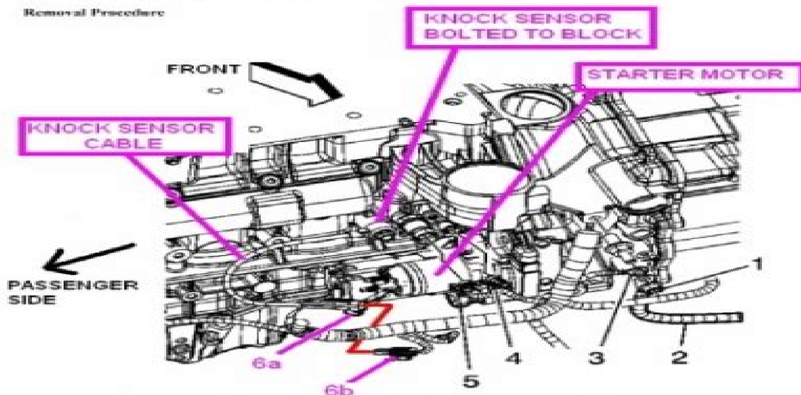
Fig. 217: KS Harness Electrical Connector
