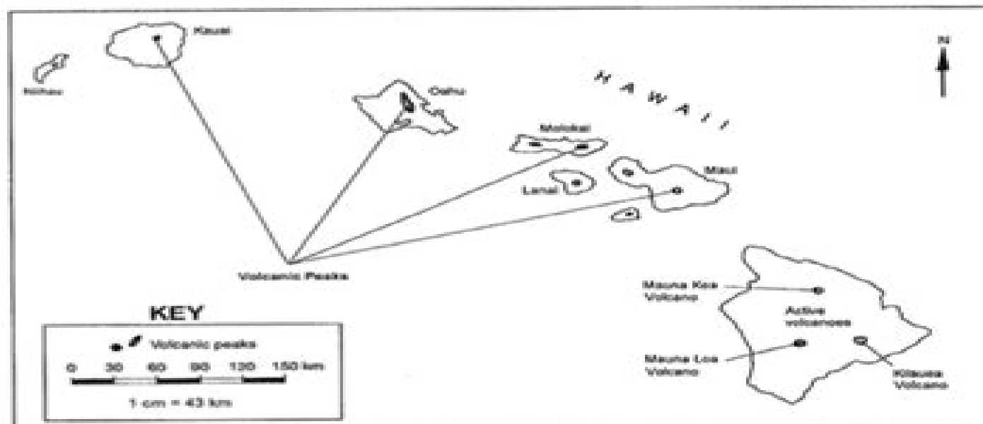
Map of the Hawaiian Islands, showing volcanic peaks. Absolute ages were determined from basalts that form the islands.
