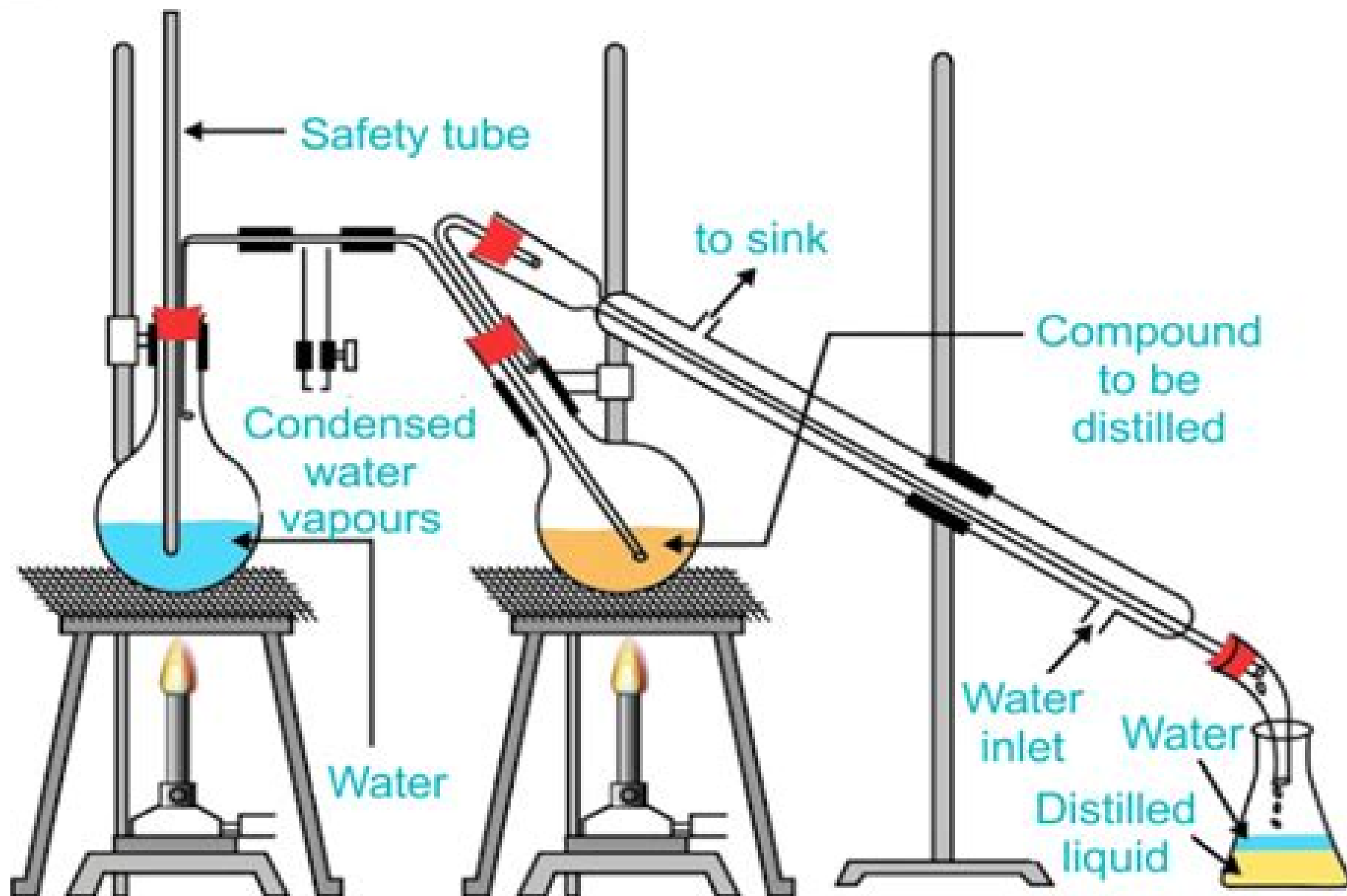
Steam Distillation
