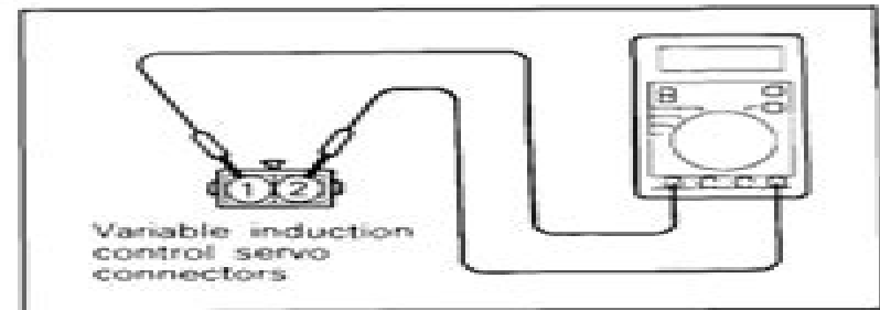
Fig. 8 — Variable intake control connector
