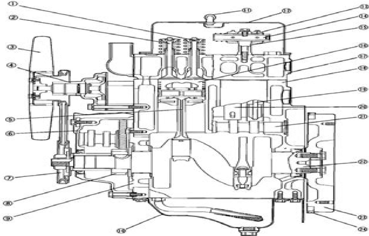
(5) Cross section of KE70
