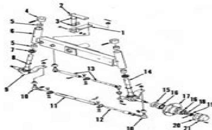
Fig. 6—Exploded view of spindles, wheel hub and steering linkage used on Model MT300.
