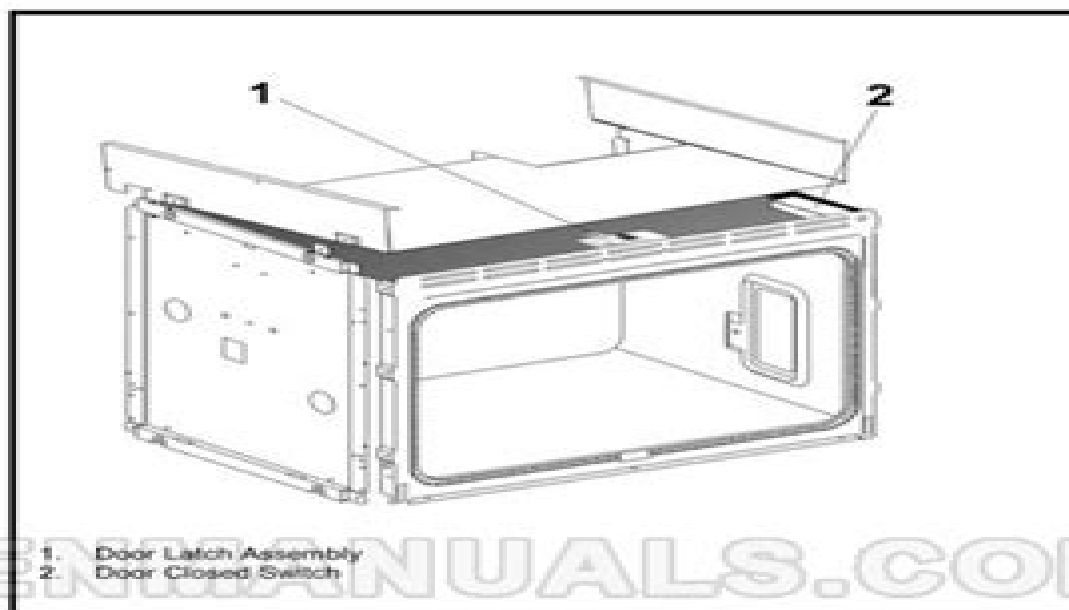
Figure 5-14: Lifting the front of the Upper Housing to access the Door Lock / Latch Assembly and Door Closed Switch
