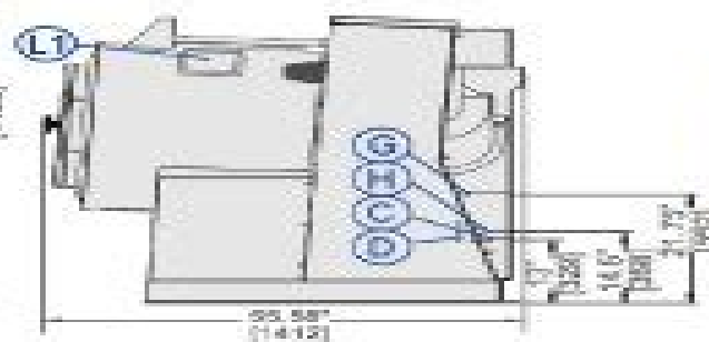
ANCHORING DETAIL
