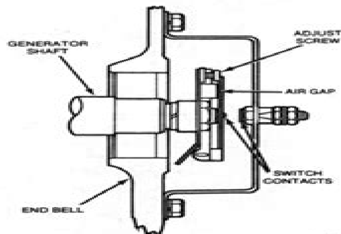
FIGURE 5-3. OPTIONAL OVERSPEED SWITCH S4
