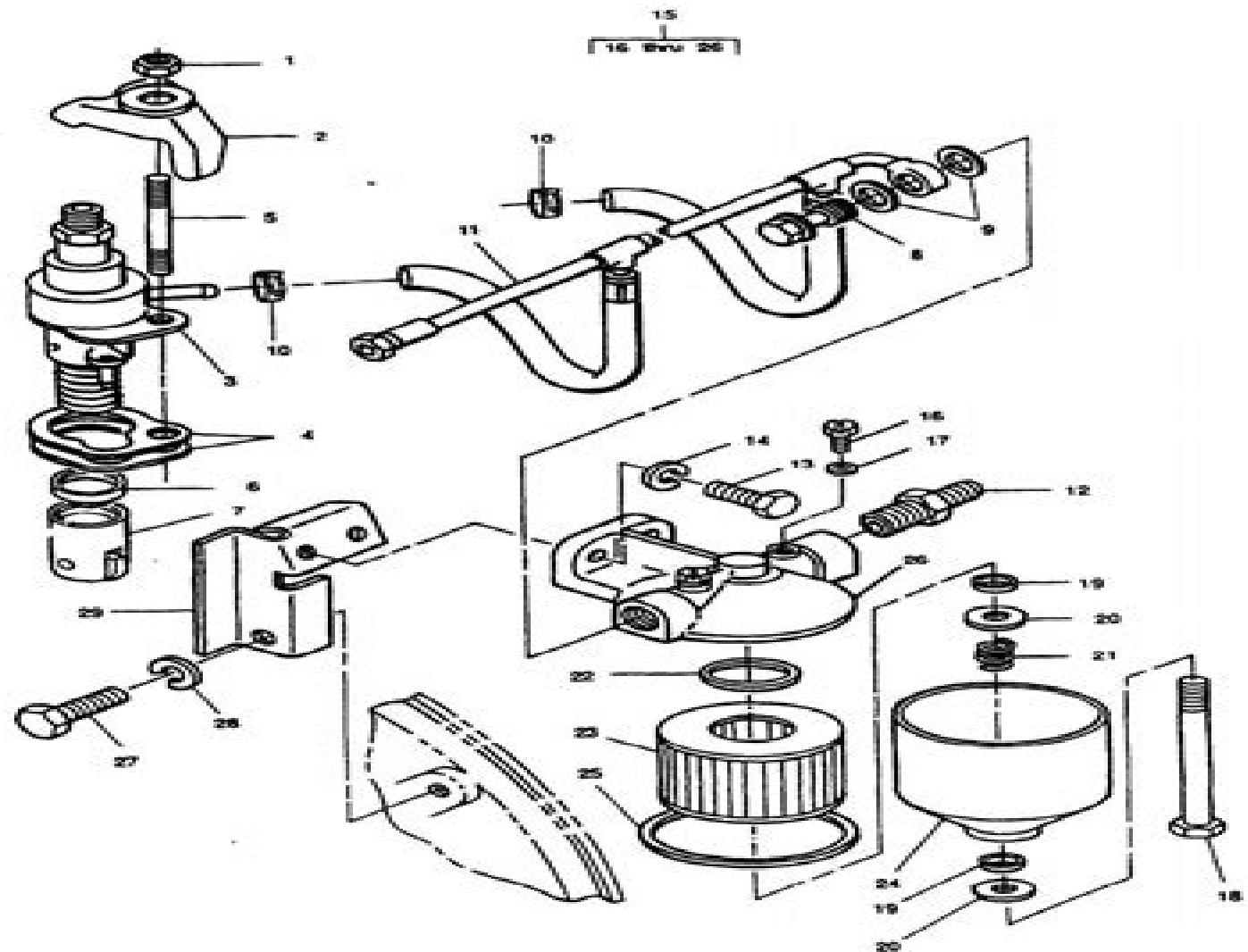
Figure 4. Fuel Pump and Lines
