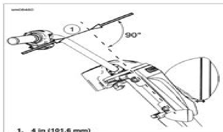
Figure 2-30. Handlebar Adjustment: FLRT
