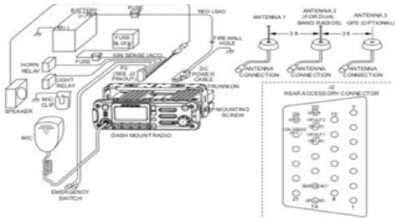
Figure 2-4. Radio Installation (O2 Mid Power Dash Mount)
