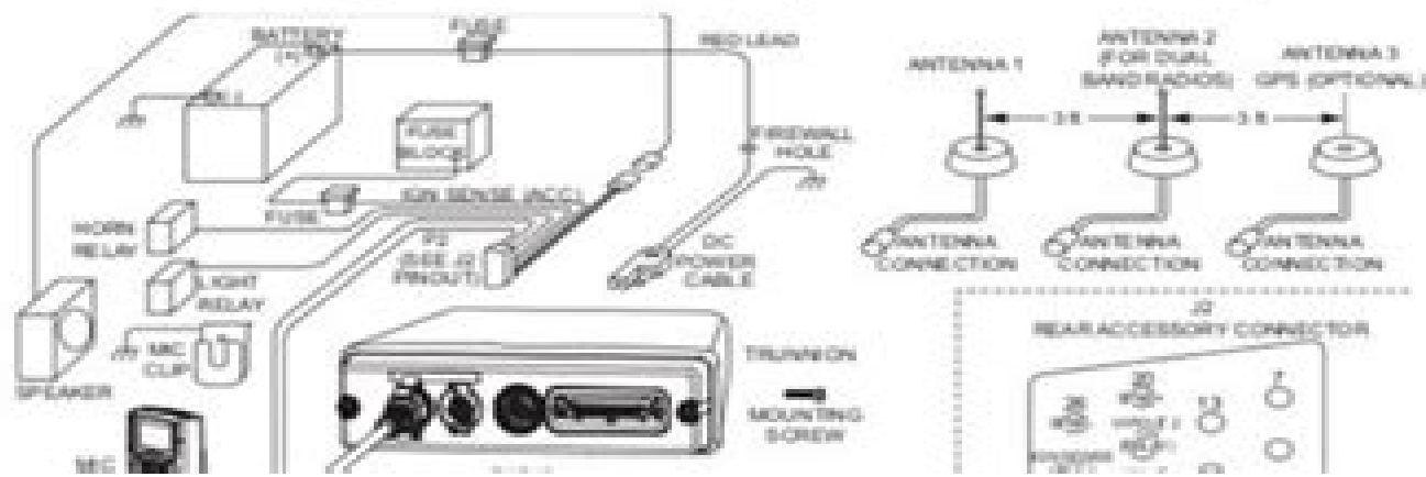
Figure 2-4. Radio Installation (O2 Mid Power Dash Mount)
