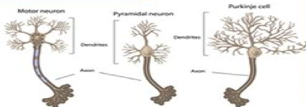
MULTIPOLAR NEURONS
