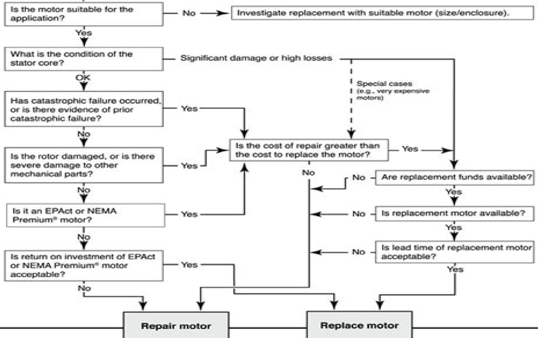
Failed motor
