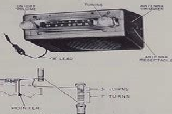
FIGURE 3. DIAL CORD RESTRAINING DETAIL
