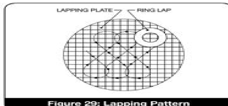
Figure 29: Lapping Pattern
