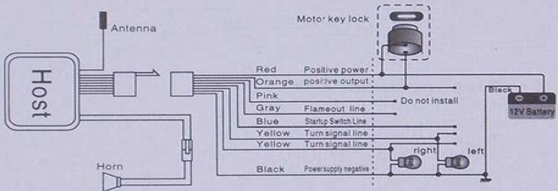
DC motorcycle ignition wiring diagram
