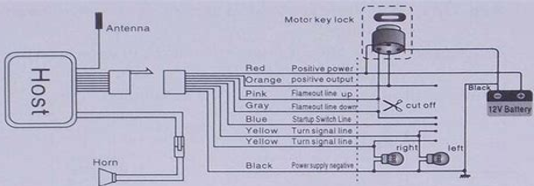
DC motorcycle ignition wiring diagram
