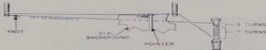
FIGURE 3. DIAL CORD RESTRAINING DETAIL
