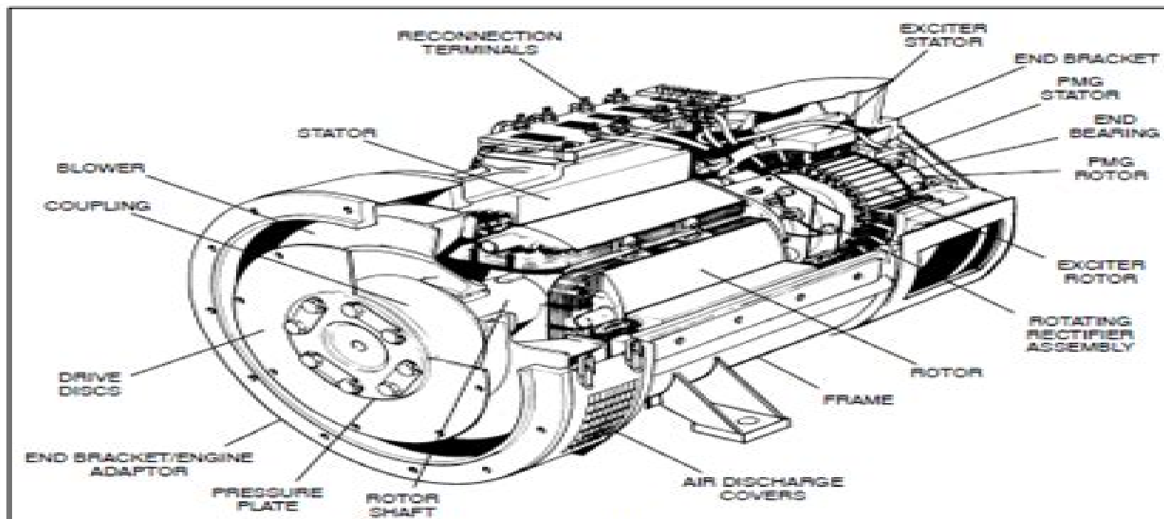
FIGURE 6-1. TYPICAL GENERATOR
