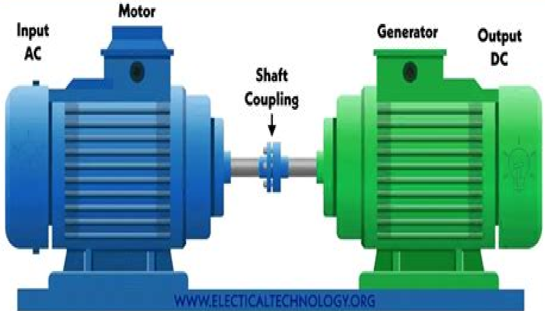
Motor-Generator Set
