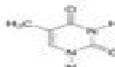
Thymine
