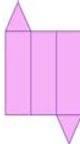
Net of a triangular prism
