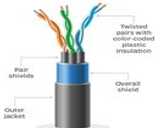
Shielded twisted pair
