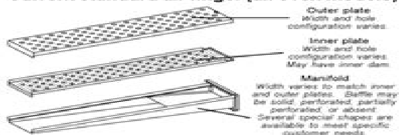
Figure 4 Current standard air finger (all oven models)
