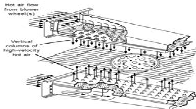
Figure 2 Air finger operation
