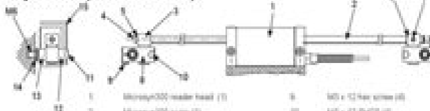
Figure 2 - Microsyn300 Encoder Assembly
