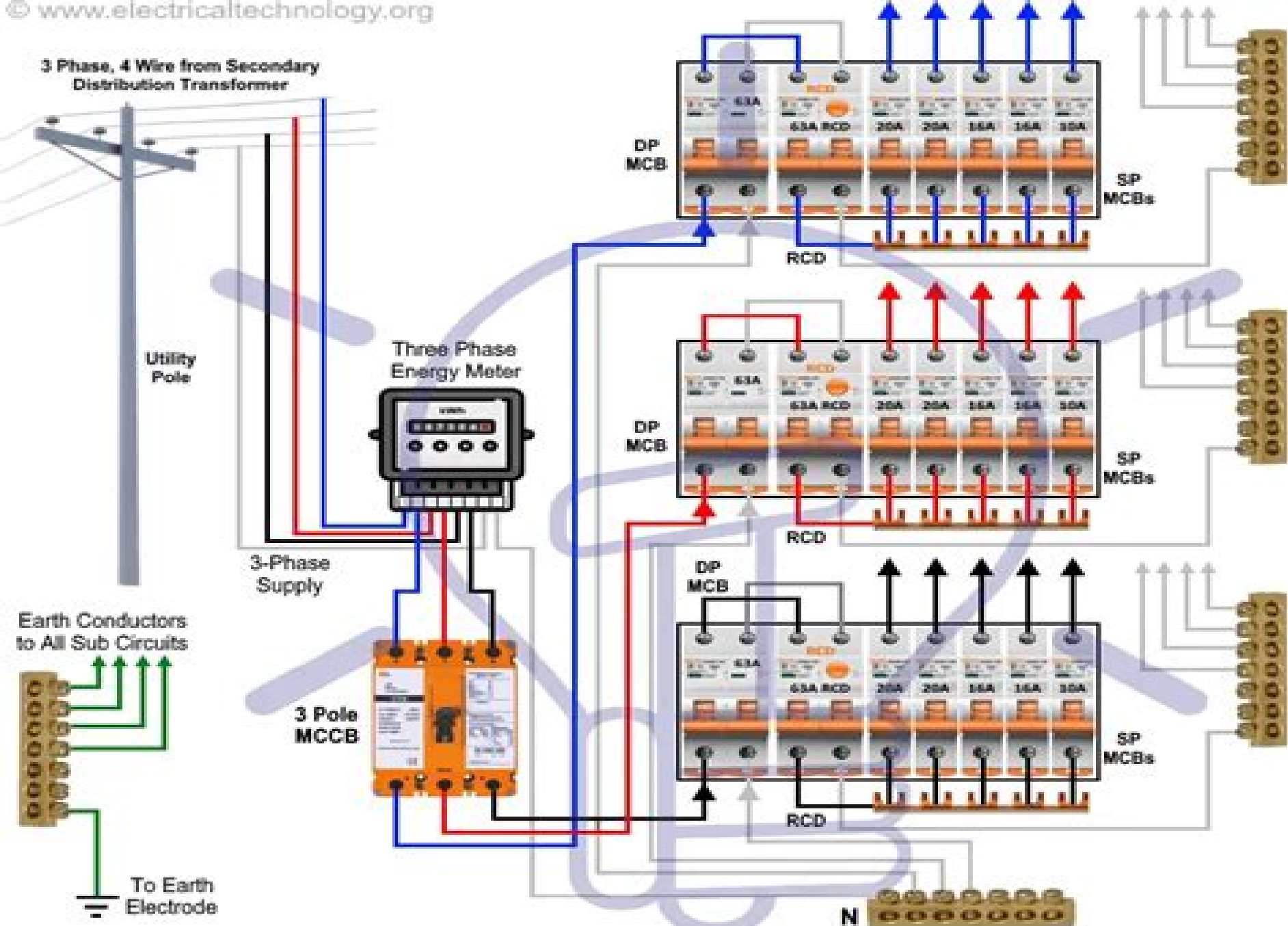
3-Phase Electrical Wiring Installation - NEC Color Code (US & Canada)
